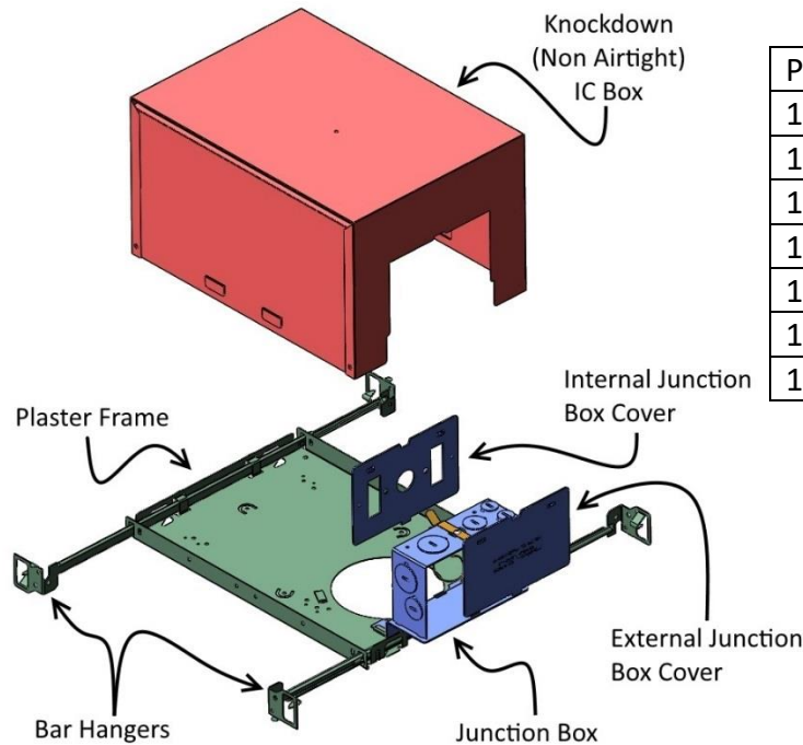
Fig. 4 Typical non-airtight IC Box placed behind plaster frame assembly containing integral junction box & junction box covers
